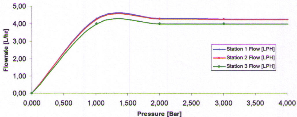
Research and Development Short Test for 4 L/h ON LINE PC DRIPPER
